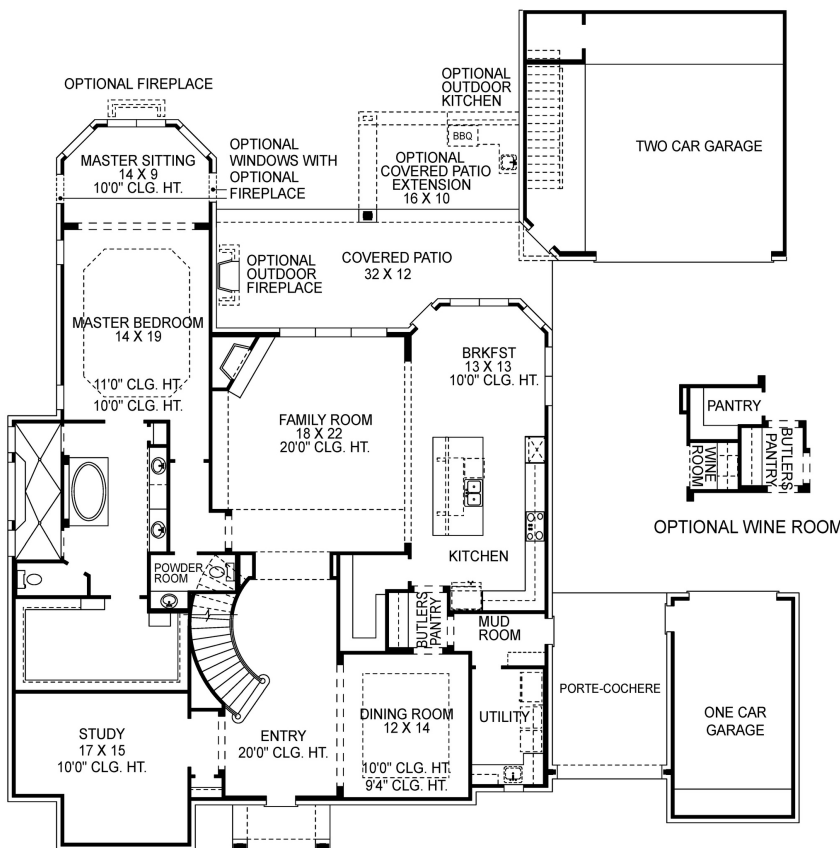
first floor
