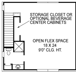
OPTIONAL SECOND FLOOR OVER TWO CAR DETACHED GARAGE
