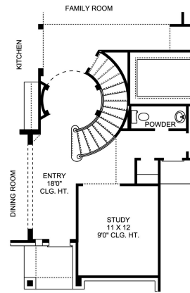
OPTIONAL CURVED STAIRCASE AT FIRST FLOOR
