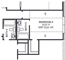
OPTIONAL BEDROOM 5 AND BATH 5 AND CLOSET IN LIEU OF MEDIA ROOM AND PART OF BEDROOM 4 CLOSET
