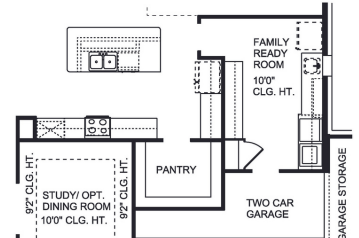
OPTIONAL READY ROOM IN LIEU OF 3RD CAR GARAGE BAY
