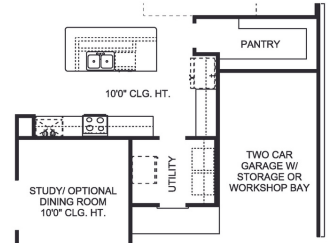
OPTIONAL KITCHEN LAYOUT WITH LARGE PANTRY
