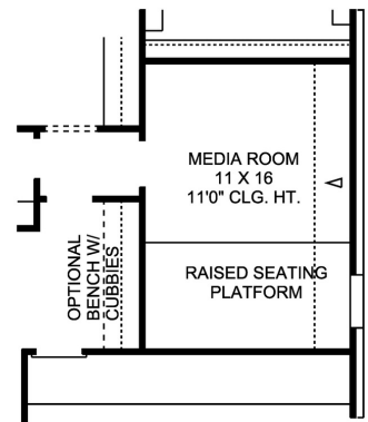
OPTIONAL MEDIA ROOM IN LIEU OF 3RD CAR TANDEM GARAGE AREA
