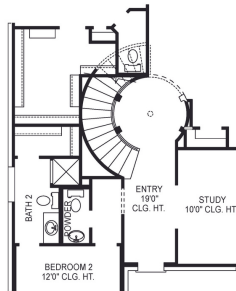
OPTIONAL ROTUNDA STAIRS FIRST FLOOR PLAN
