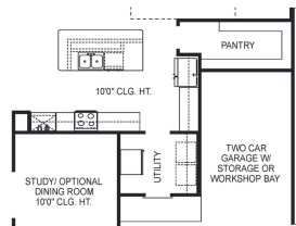
OPTIONAL KITCHEN LAYOUT WITH LARGE PANTRY
