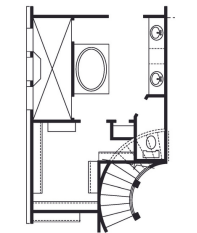
OPTIONAL ROTUNDA STAIRS W/ OPTIONAL MASTER BATH AT FIRST FLOOR
