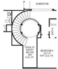
OPTIONAL ROTUNDA STAIRS SECOND FLOOR PLAN
