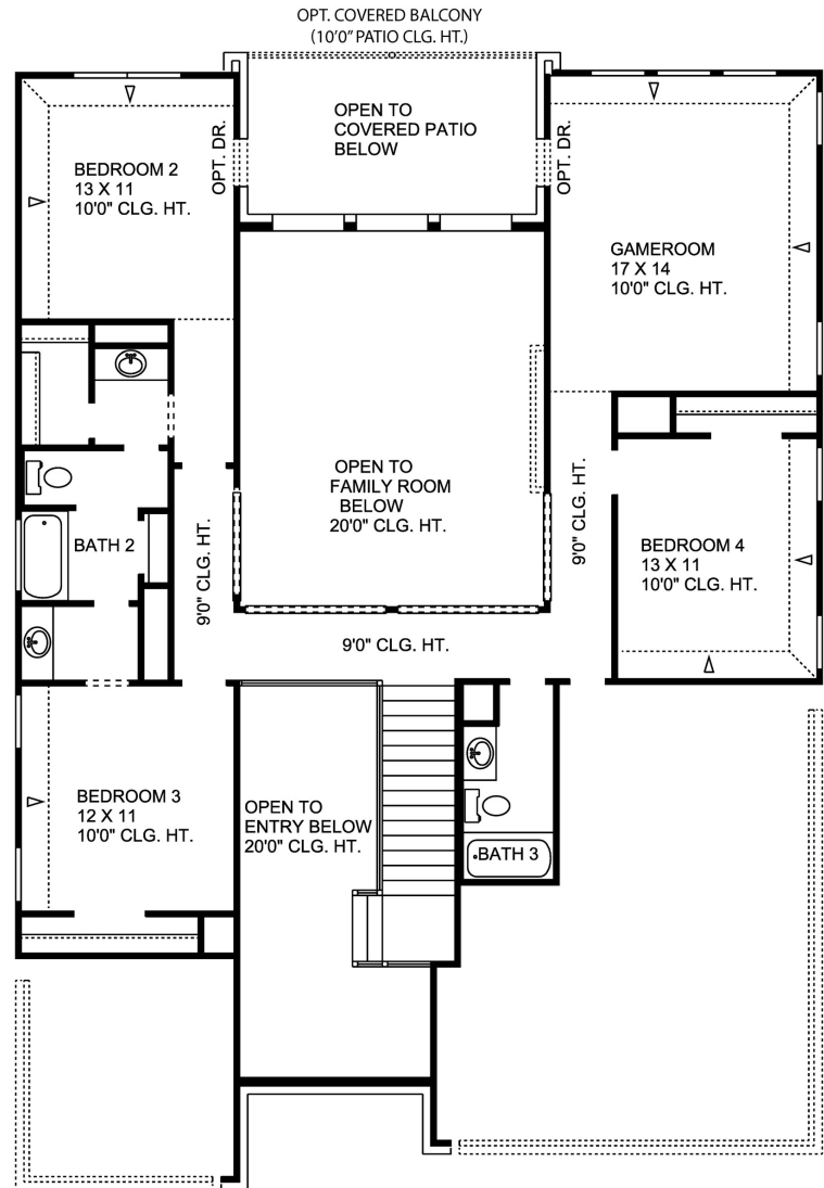
second floor
