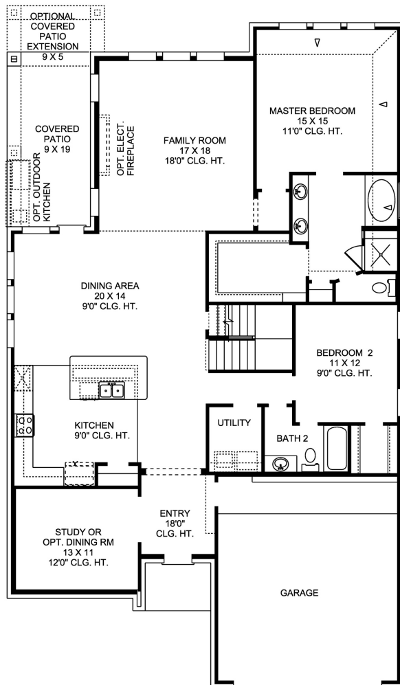
OPTIONAL PREFAB. FIREPLACE AT FAMILY ROOM
