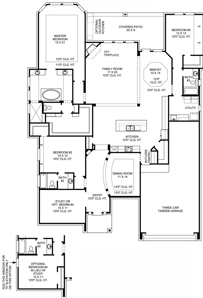
floor plan
